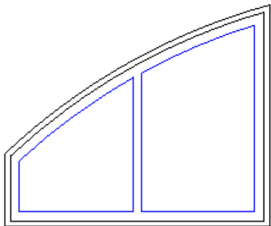
As Viewed From The Exterior FS 28" X 22 51/64" RO 29" X 23 7/16" Egress Information No Egress Information available.
