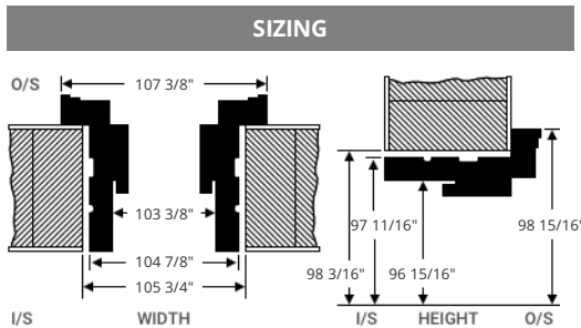
OUTSIDE VIEW
