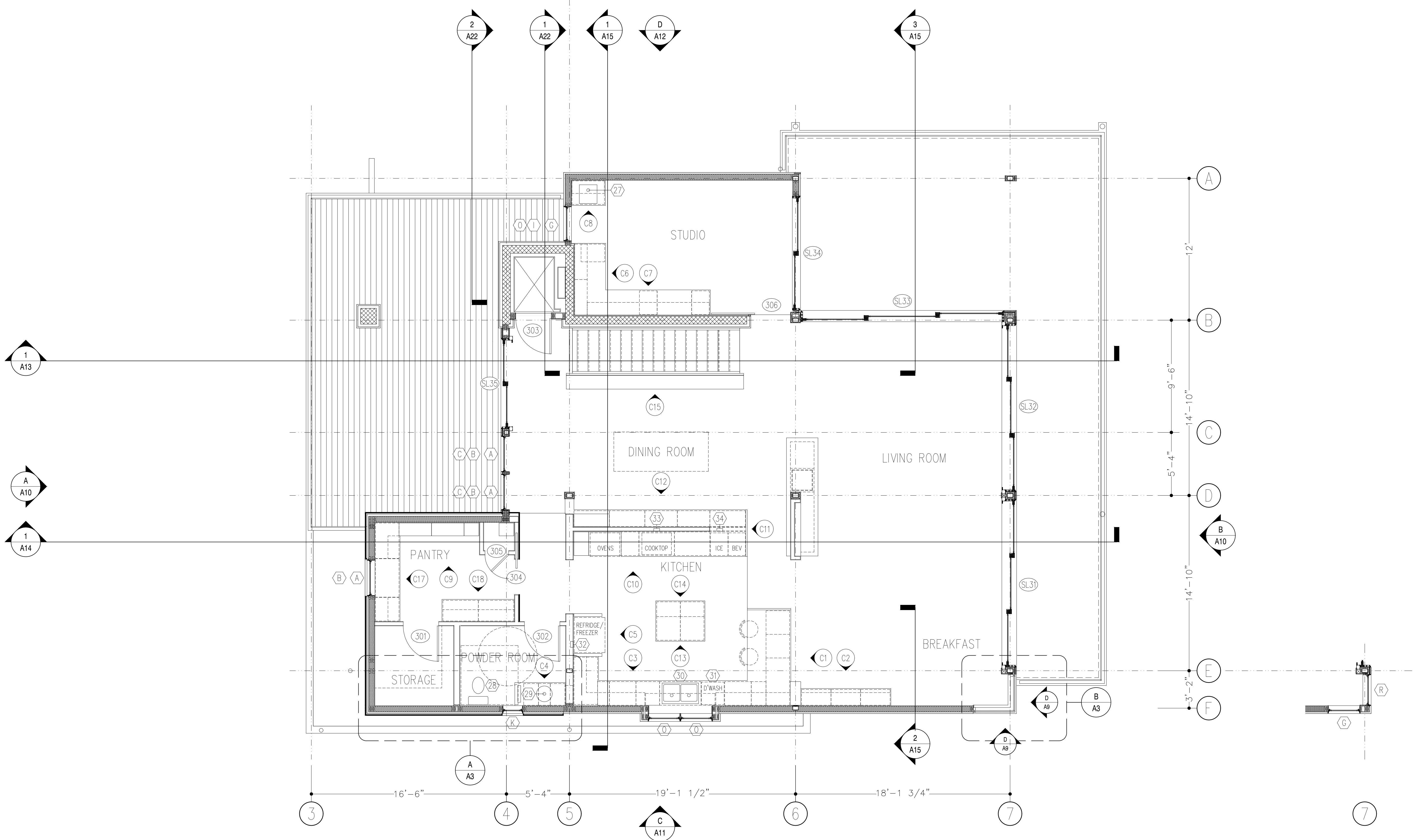
3rd FLOOR PLAN
