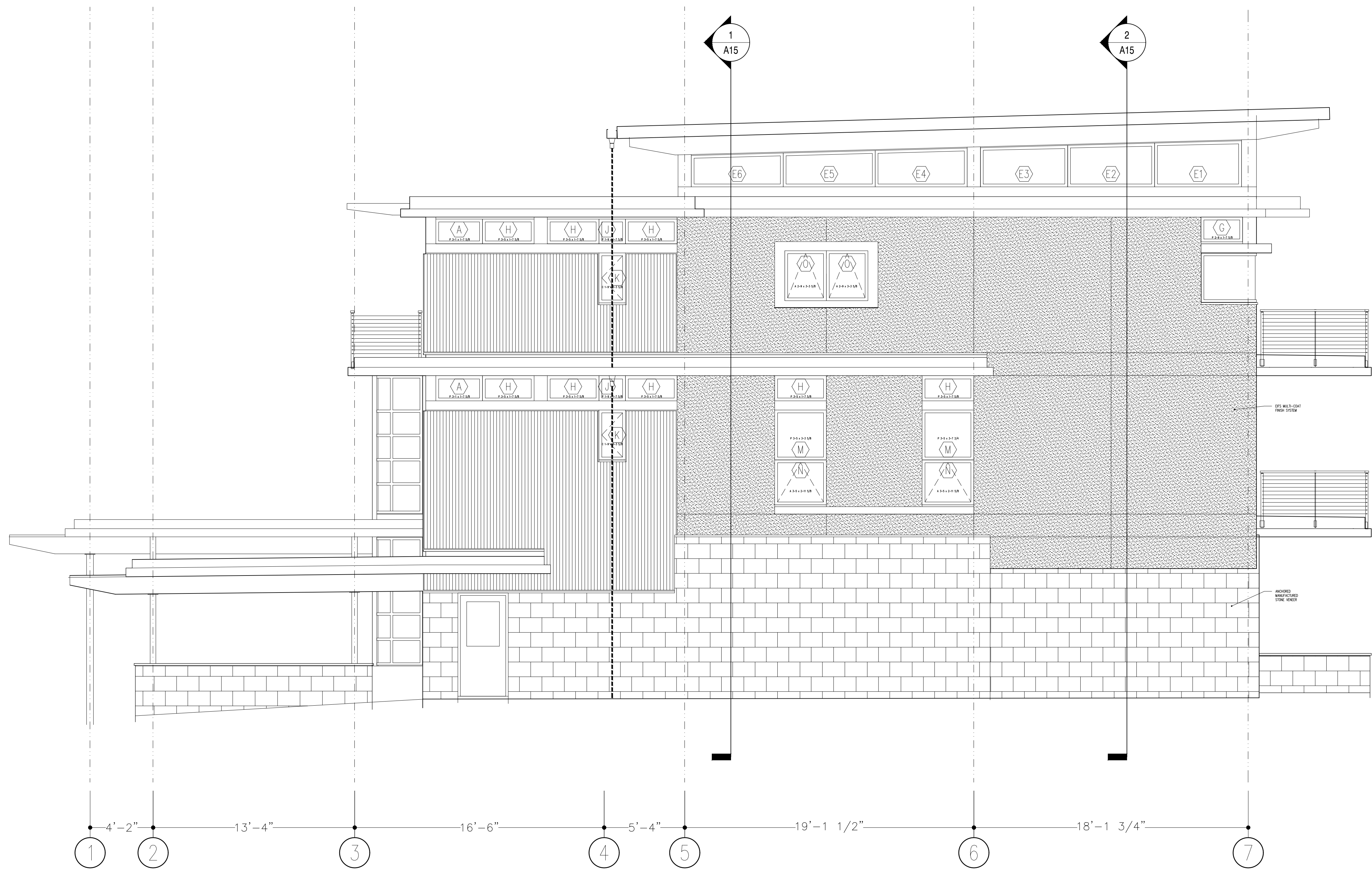
C A11 EAST ELEVATION
