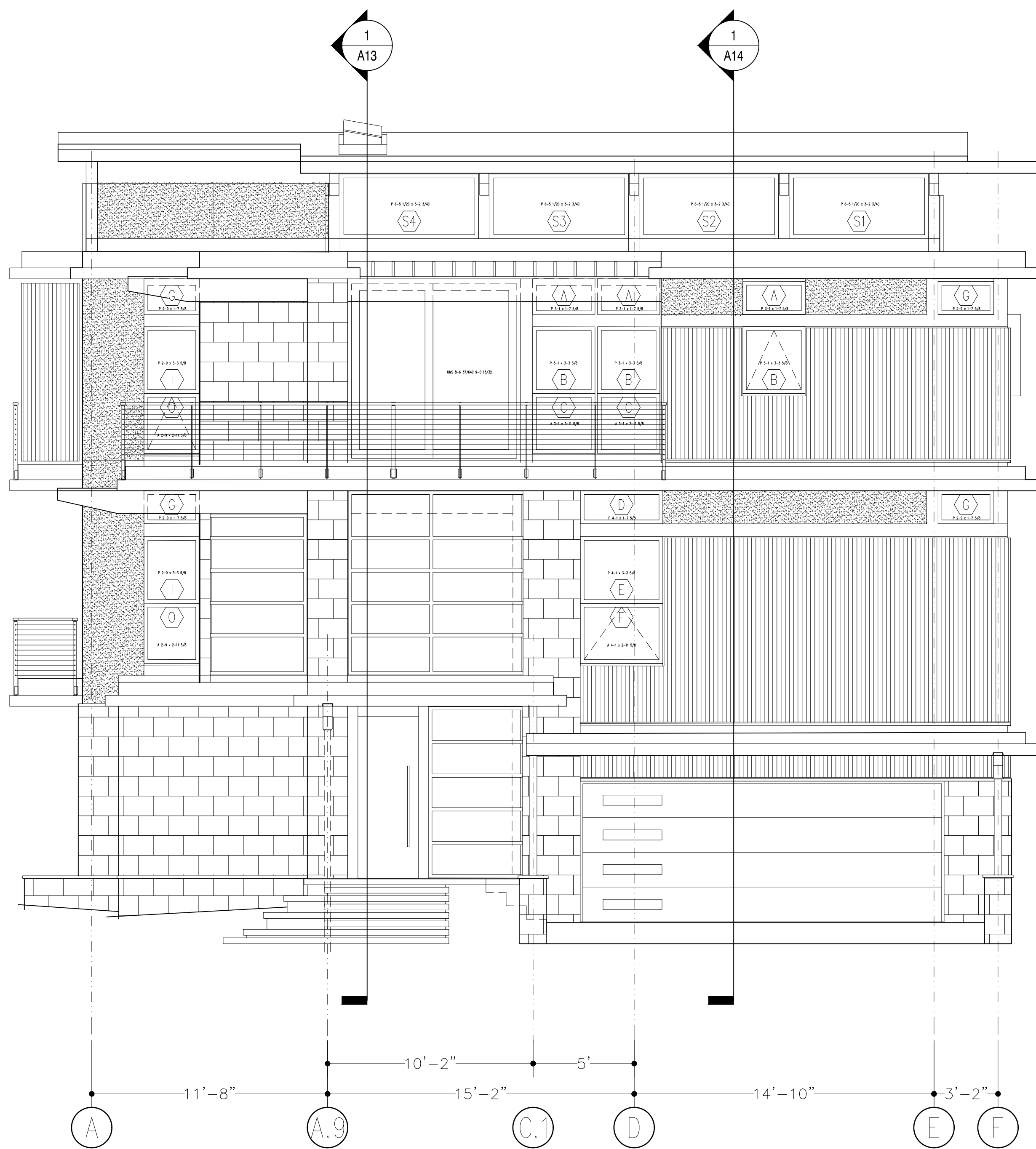
A SOUTH ELEVATION A10
