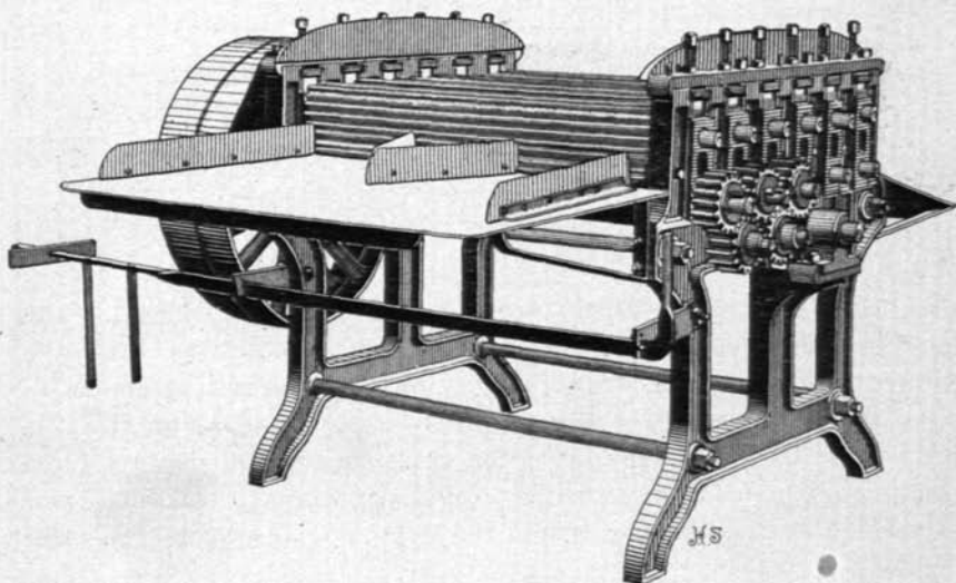
FIG. 7.—Typical flax-fiber breaking machine.
